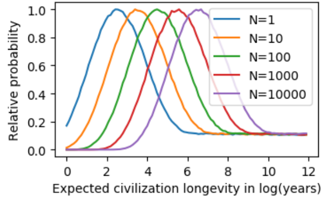
Figure 1: Graph for \log(L) , i.e. for expected human longevity based on the values of N - the number of civilizations in our galaxy.
