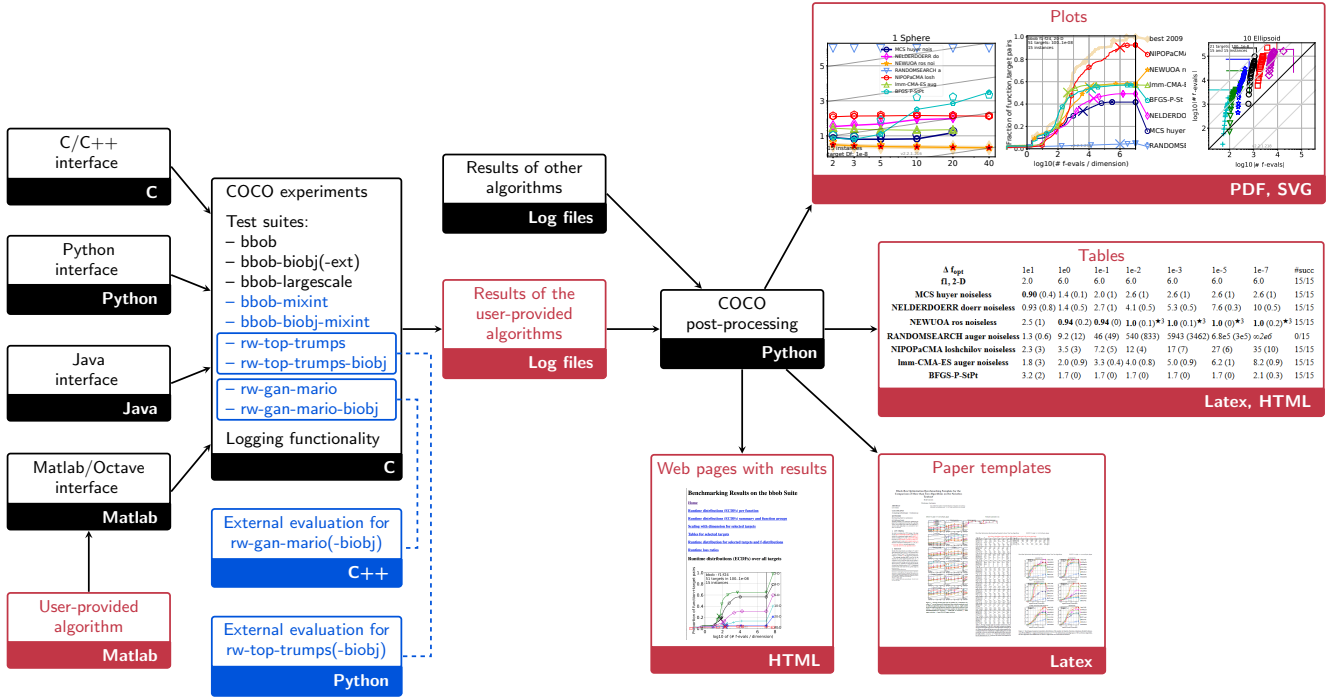
Figure 1: The COCO platform scheme. Its main components are presented in black, while the user-provided algorithm and its results are shown in red. Blue color is used to denote the recent additions.
